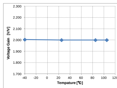
Voltage Gain
